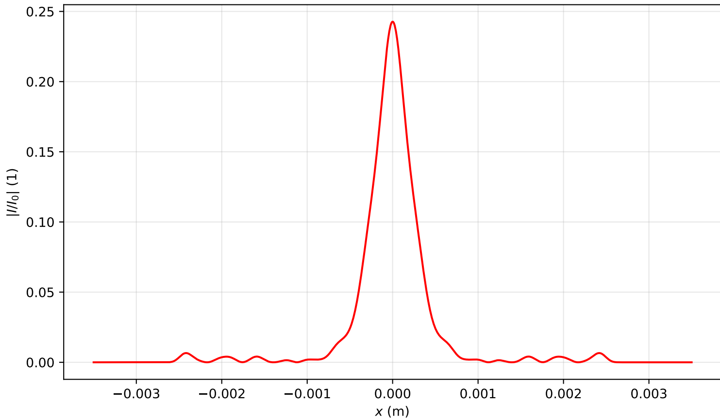
Intensity profile I(x, y = 0, z = 2.548)/I_0 , \text{Pin}=6.0\text{Pcr} , artificial time
